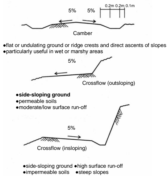
Figure 3: Typical cross-sections for improved paths and tracks
