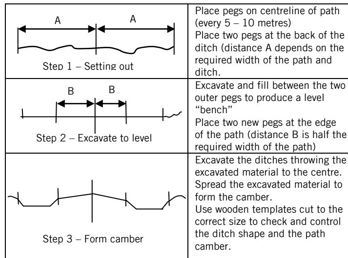
Figure 5: Construction sequence
