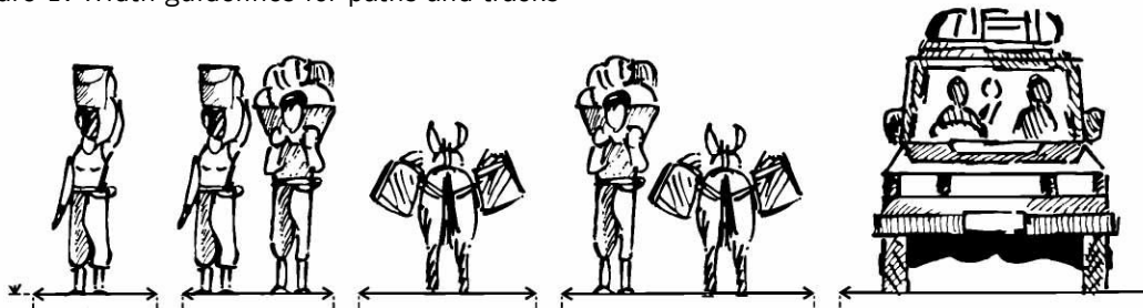
Figure 1: Width guidelines for paths and tracks
